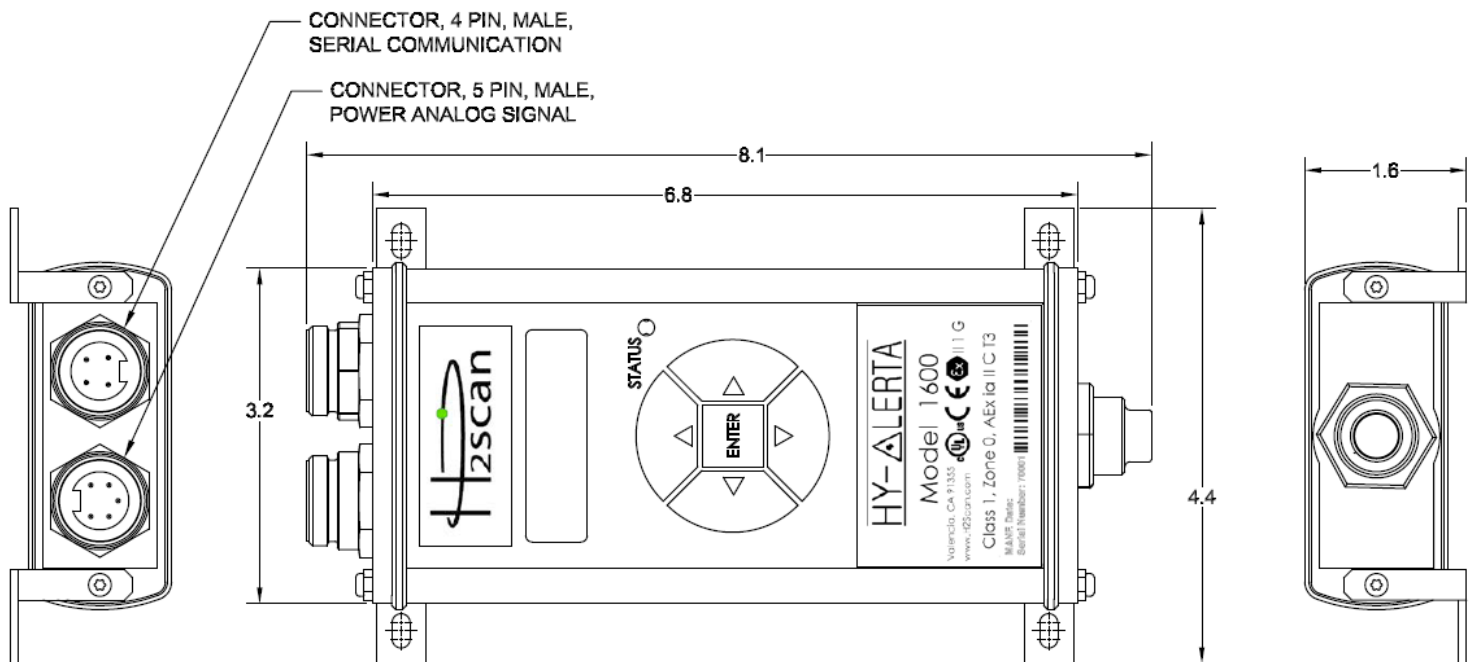
Figure 2: Dimensions (inches)
